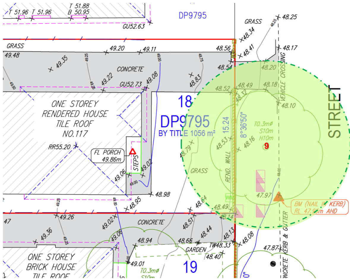
Fig 2: Survey/ Subdivision- Tree locations (1-10)
